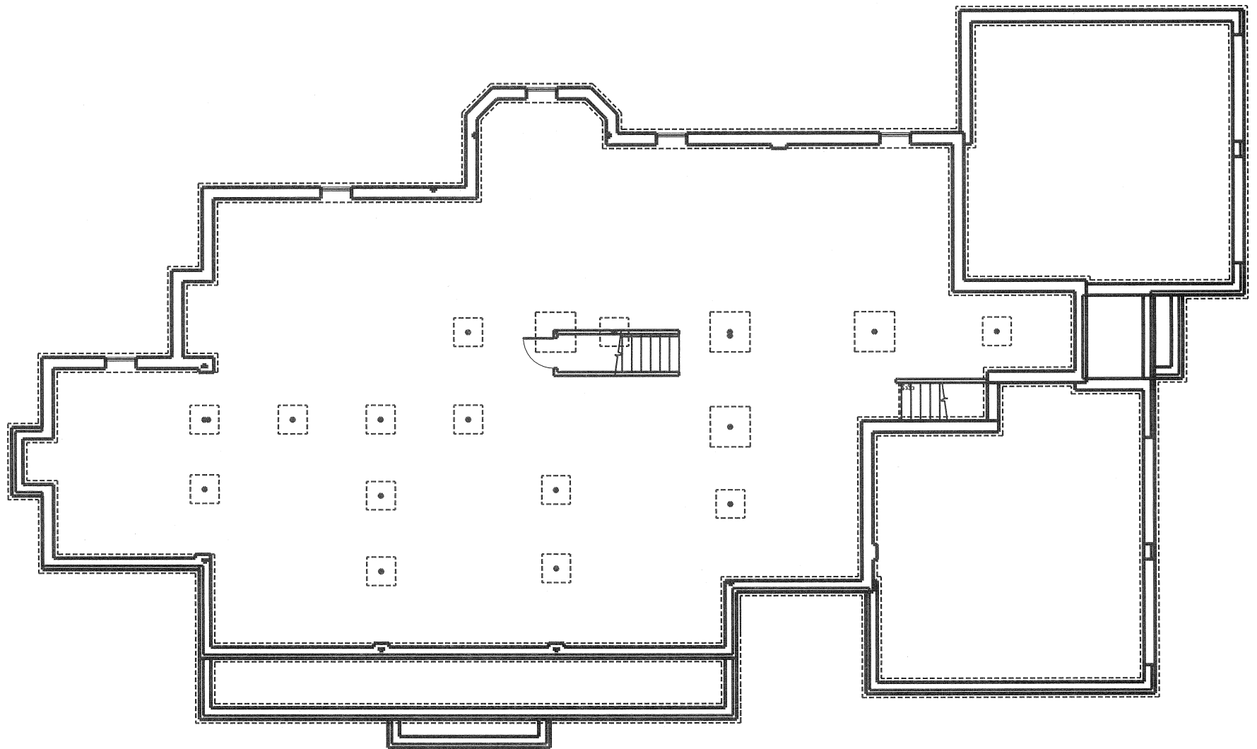
BASEMENT PLAN NOT TO SCALE
